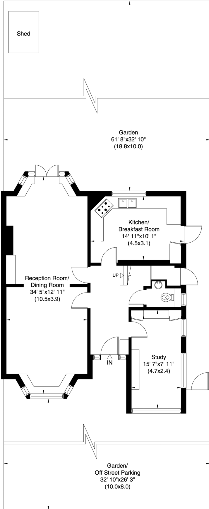
Ground Floor
