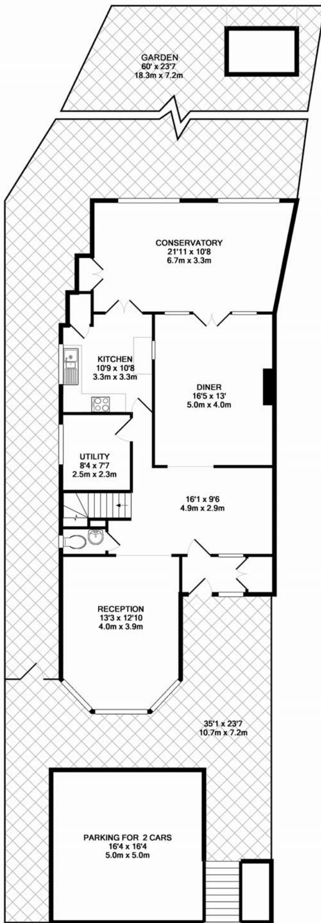
GROUND FLOOR APPROX. FLOOR AREA 134.3 SQ.M. (1446 SQ.FT.)
