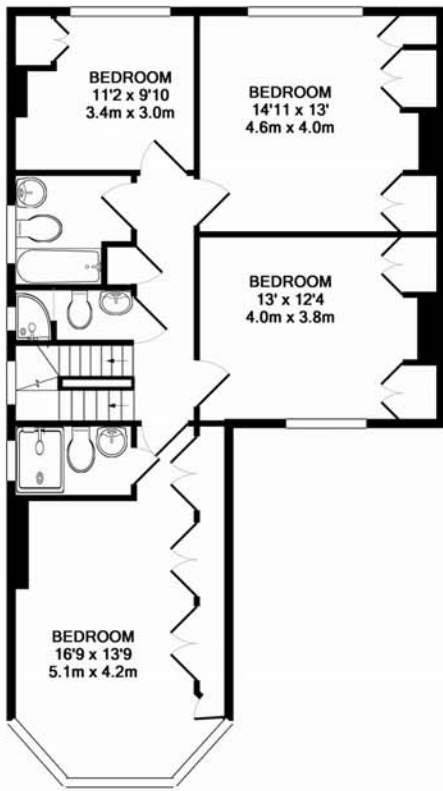
1ST FLOOR APPROX. FLOOR AREA 64.9 SQ.M. (699 SQ.FT.)
